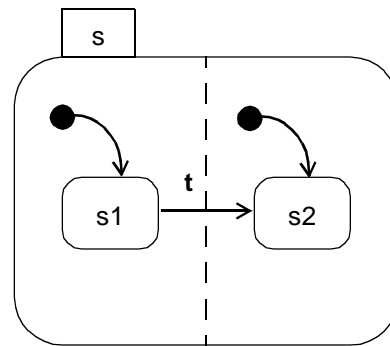
Figure 2-23 Unstructured transition among regions
