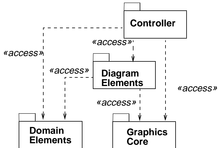
Figure 3-42 Dependencies Among Packages
