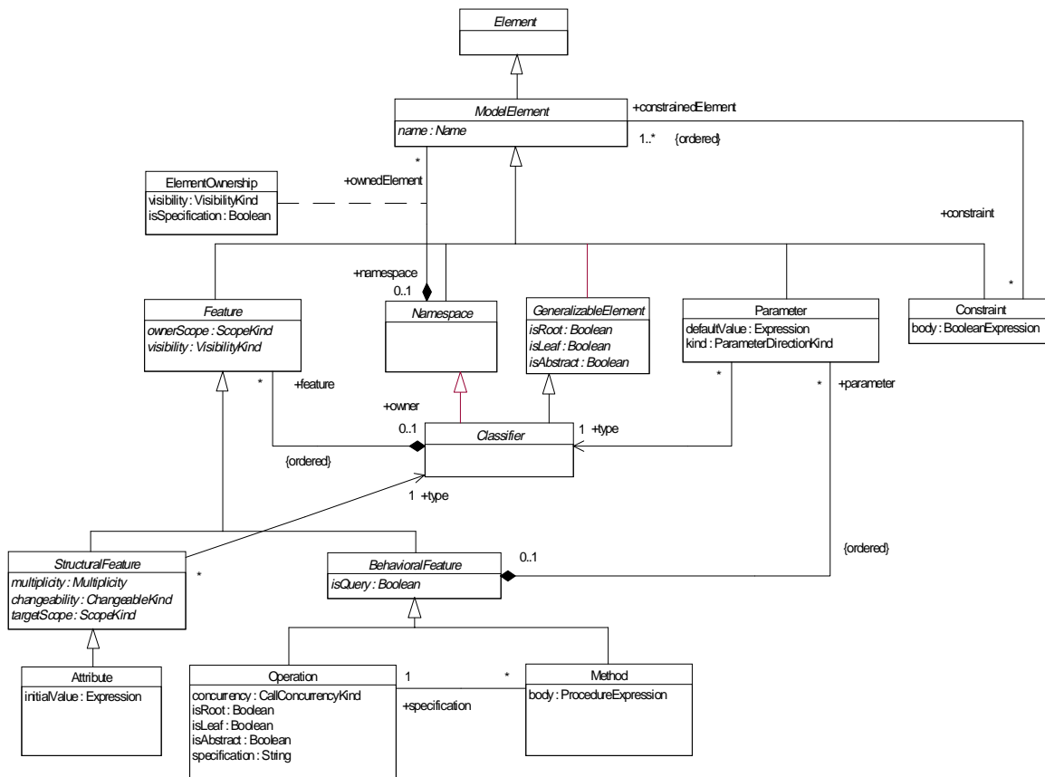
Figure 2-5 Core Package - Backbone
