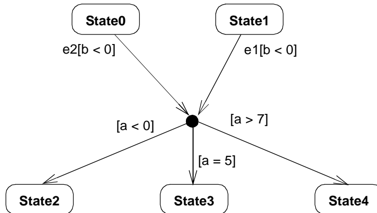
Figure 3-68 Junction points
