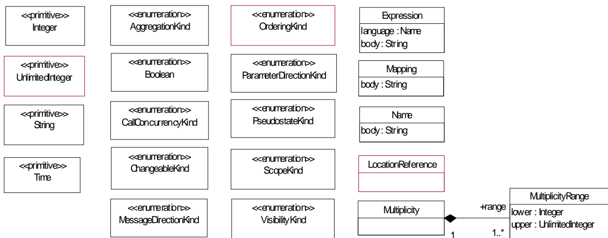
Figure 2-11 Data Types Package - Main
